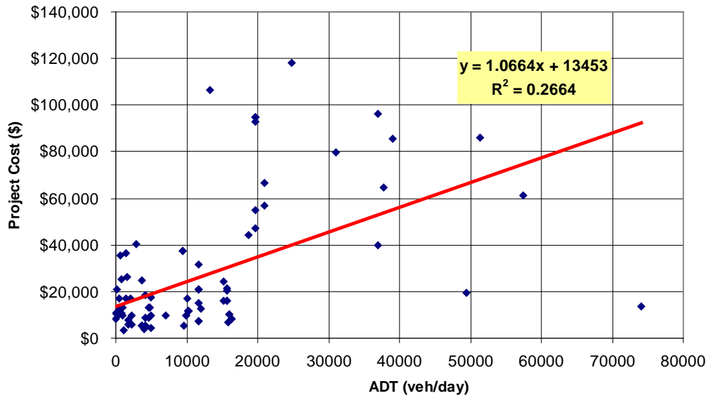
Figure 5.14. Variation in bridge minor rehabilitation project costs relative to Average Daily Traffic (ADT)
