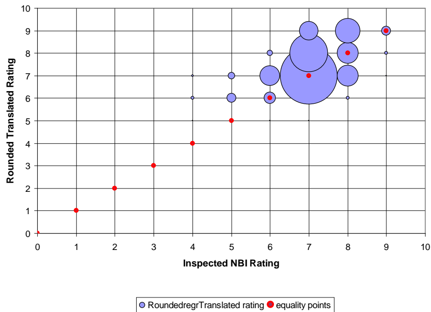
Figure 3.19. Bubble plot for variation in rounded regression-modified translated ratings for decks on state-maintained bridges inspected in 2008.
