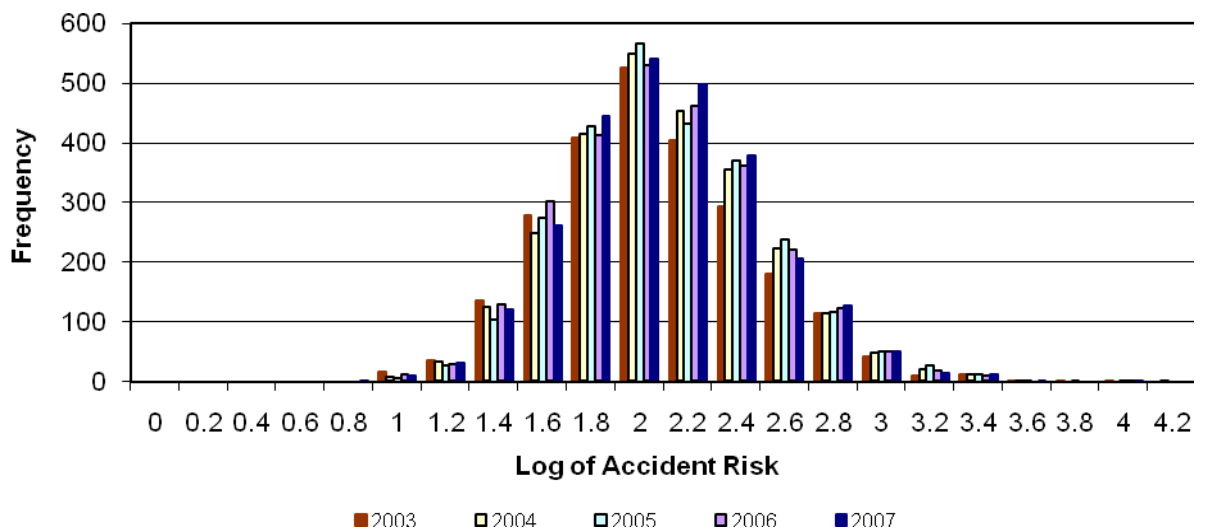
Figure 6.21. Frequency distribution of log accident risk 2003-2007
