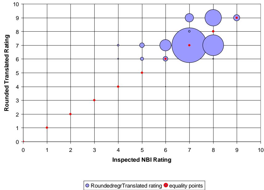
Figure 3.20. Bubble plot for variation in rounded regression-modified translated ratings for superstructures on state-maintained bridges inspected in 2008
