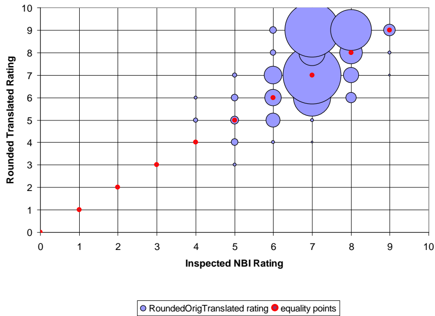
Figure 3.18. Bubble plot for variation in rounded original translated ratings for decks on state-maintained bridges inspected in 2008
