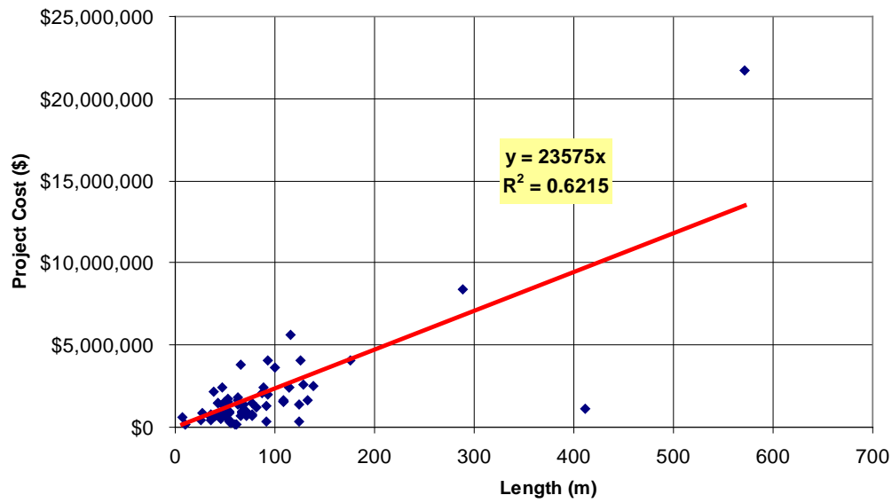
Figure 5.16. Variation in bridge widening project costs relative to bridge length
