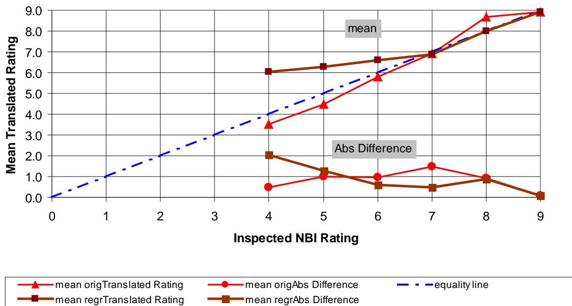
Figure 3.17. Variation in translated ratings for culverts inspected in 2008 on state-maintained bridges
